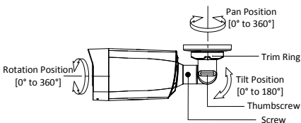
Figure 2-2 3-Axis Adjustment
