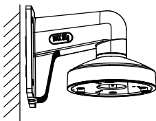
Figure 2-13 Fix the Wall Mount
