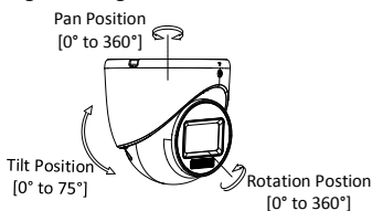
Figure 2-9 3-Axis Adjustment
