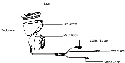
Figure 1-5 Overview of Type V Camera
