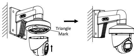
Figure 2-16 Finish Installation
