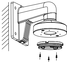
Figure 2-15 Fix the Base
