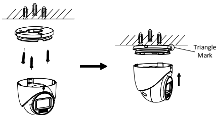
Figure 2-8 Install the Camera to Ceiling
