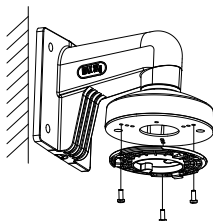
Figure 2-14 Fix the Installation Plate
