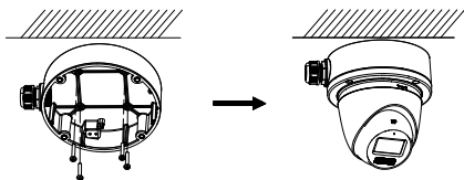
Figure 2-11 Fix the Junction Box Cover and Junction Box Body
