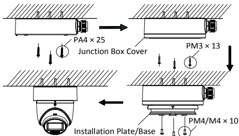
Figure 2-12 Fix the Camera to the Junction Box
